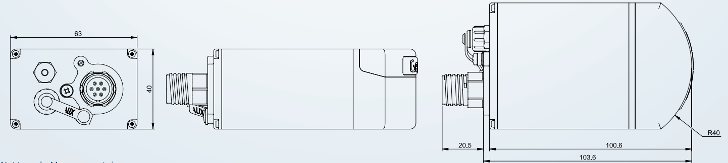
Not to scale. Measurements in mm
