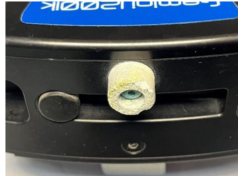
Used anode, approx. 80% of original size.
