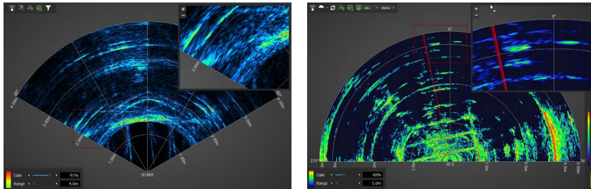
Multibeam (left) and Scanning (right) Sonar displays with Acoustic Zoom active.
