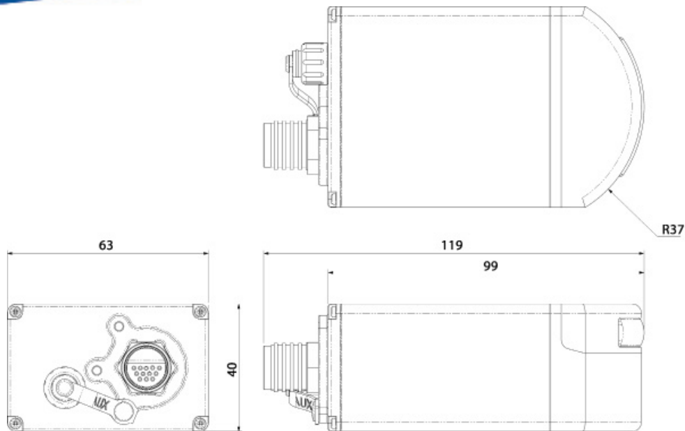
Drawing shown with Seacon connector. All dimensions are in mm, not to scale
